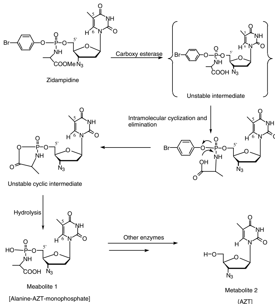
Scheme 1. Proposed hydrolysis pathway of Zidampidine in vivo .
