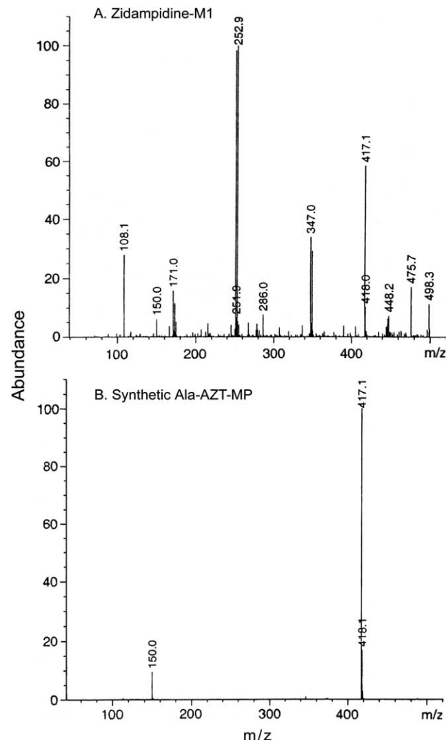
Figure 2. Mass spectra of Zidampidine-M1 obtained from plasma extraction (A) and synthetic Ala-AZT-MP: (A) corresponds to the material extracted from the plasma after iv injection of Zidampidine and (B) represents the authentic synthetic sample of Ala-AZT-MP. The material obtained from the plasma shows complexity in the pattern perhaps due to the presence of other unknown material that eluted with Zidampidine-M1. Our intent was not to identify all the peaks from the plasma sample, but was instead to compare the peaks in the spectrum corresponding to the authentic sample of Ala-AZT-MP.
