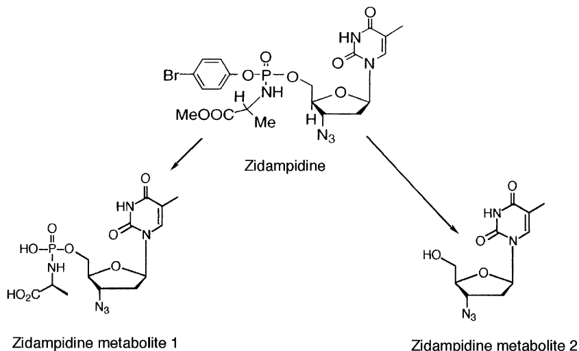
Figure 5. Metabolic pathway of Zidampidine (3'-azidothymidine-5'-[p-bromophenyl methoxyalaninyl phosphate]). Zidampidine-M1 (Ala-AZT-MP = 3'-azido-3'-deoxythymidine-5'-methoxyalaninyl phosphate) and Zidampidine-M2 (AZT = 3'-azido-3'-deoxythymidine).
