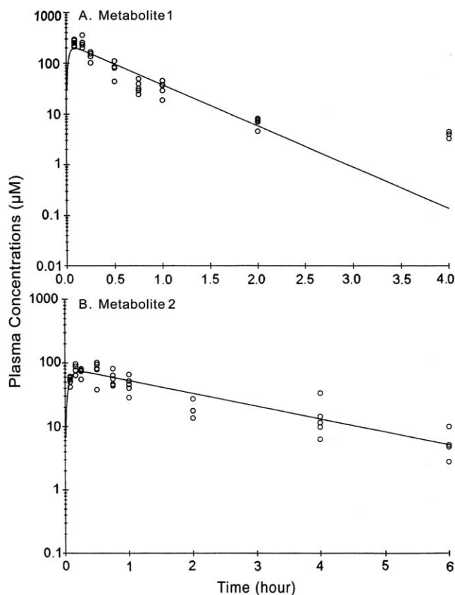
Figure 1. Plasma concentration–time profiles of Zidampidine-M1 (A) and Zidampidine-M2 (B) in CD-1 mice following iv bolus injection of Zidampidine at dose of 240/kg (five mice per time point).
