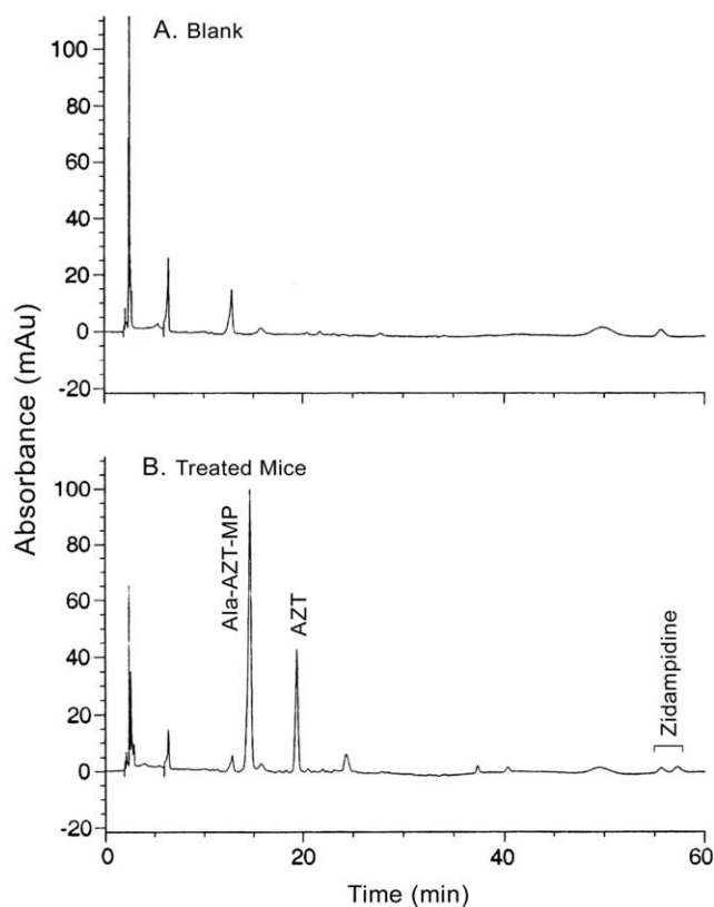
Figure 3. Representative HPLC chromatograms of blank plasma (A) and plasma sample at 10 min following iv injection 240 mg/kg Zidampidine.
